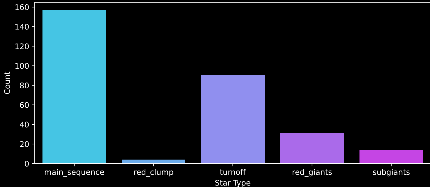
GALAH DR4 Field: [95] Count plot of Star Type
