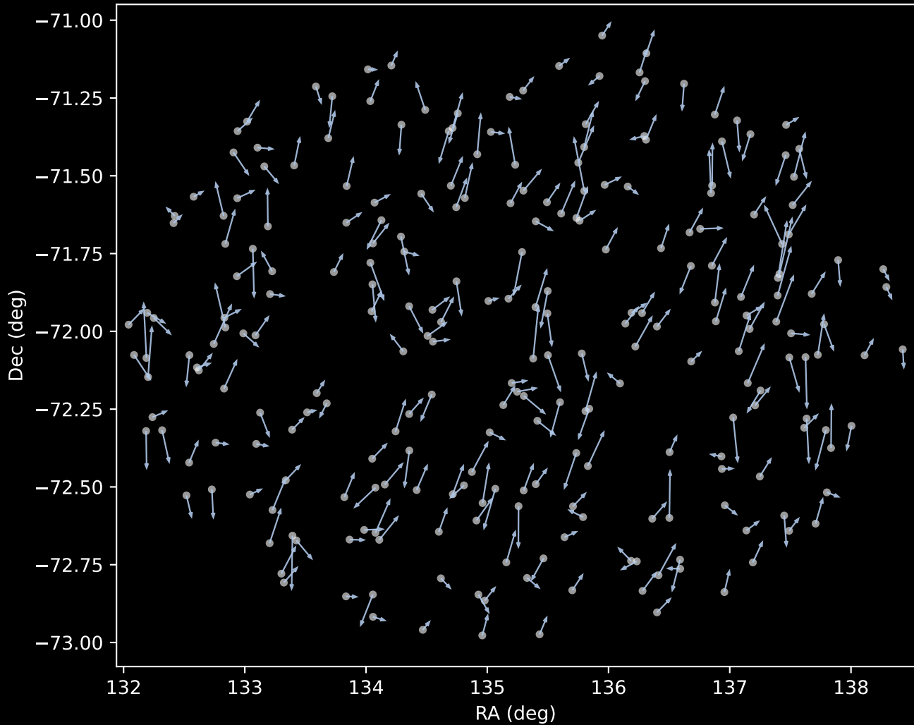
GALAH DR4 Cluster 1 Proper Motion Vectors (n=250)
