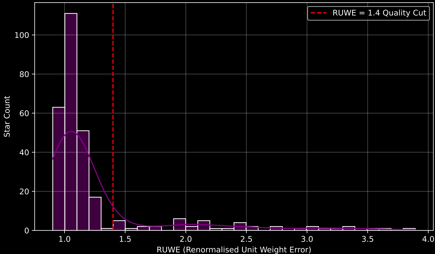
GALAH DR4 Field [95] RUWE Distribution (n= 286)
