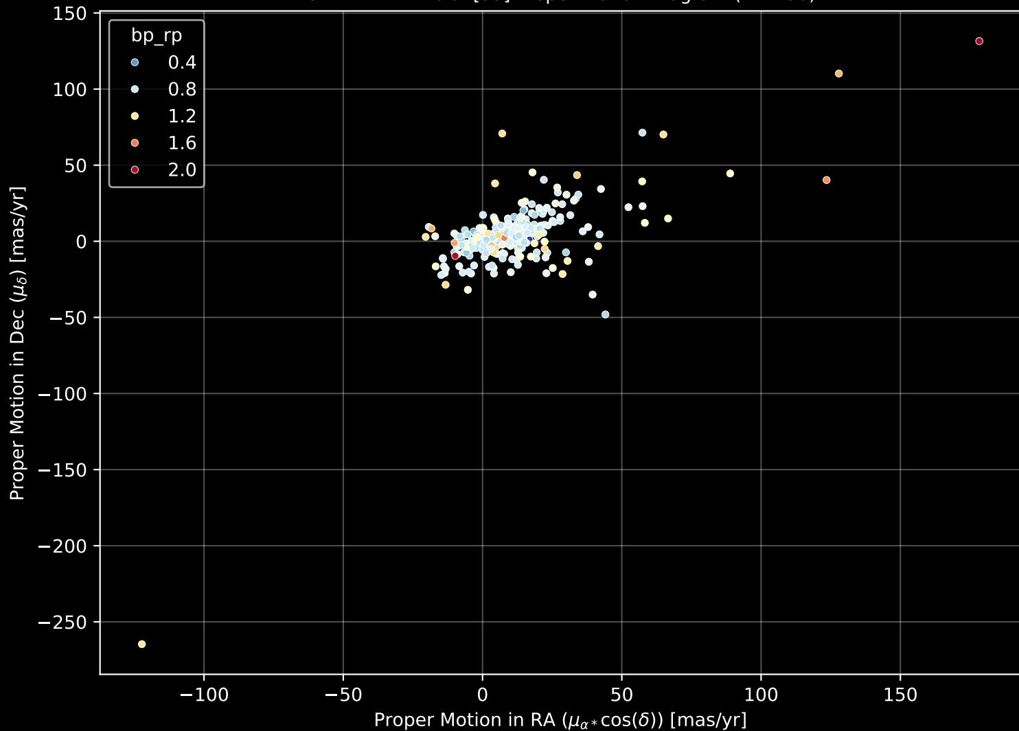
GALAH DR4 Field: [95] Proper Motion Diagram (n= 296)
